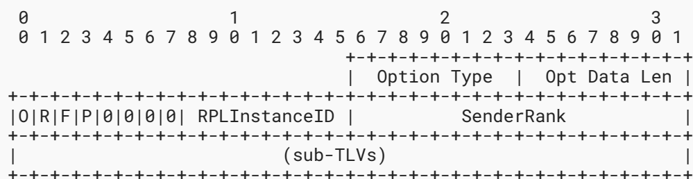
Figure 11: Amended RPL Option Format
