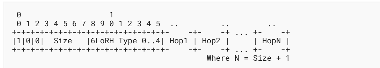
Figure 22: The SRH-6LoRH Header
