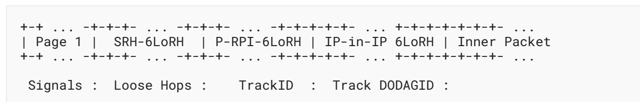
Figure 23: A Packet as Forwarded Along a Track
